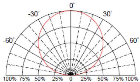
Fig.6 Directive Radiation
