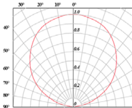
Radiation Pattern
