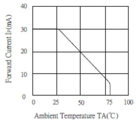
MAX FORWARD CURRENT Vs. AMBIENT TEMPERATURE
