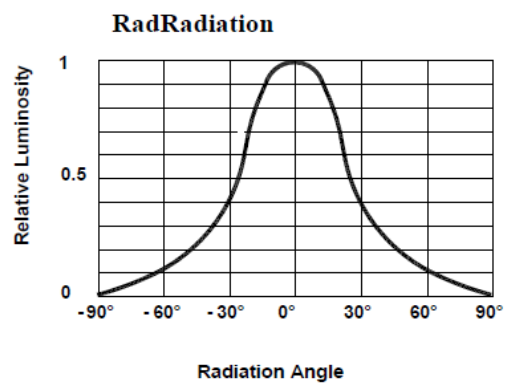
Fig6. Relative Luminous Intensity Vs.
