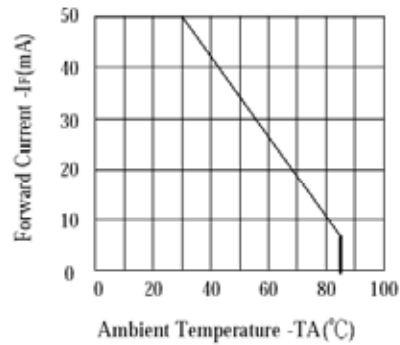
MAX FORWARD CURRENT Vs. AMBIENT TEMPERATURE
