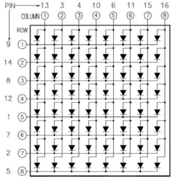
CDMA8823 SERIES (COLUMN ANODE)
