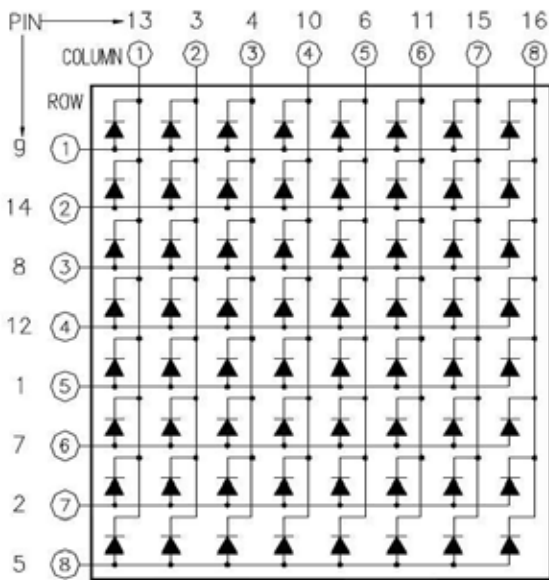
CDMC8823 SERIES (COLUMN CATHODE)
