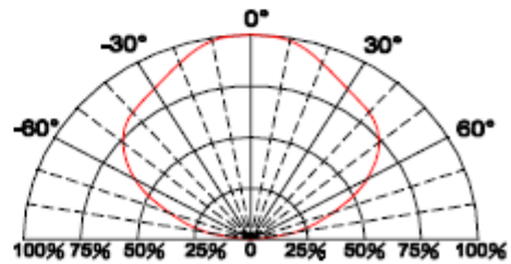
Fig.6 Directive Radiation
