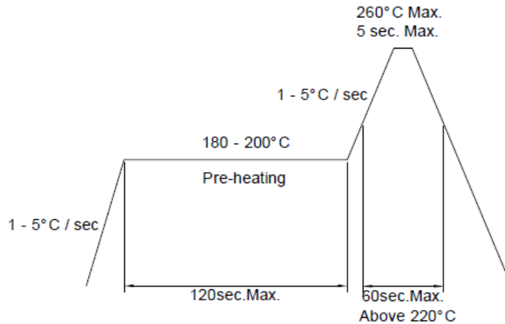
Reflow Temp/Time(Pb-free)
