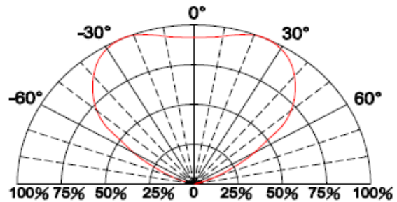
Fig.6 Directive Radiation
