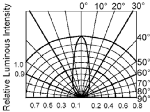
RADIATION DIAGRAM
