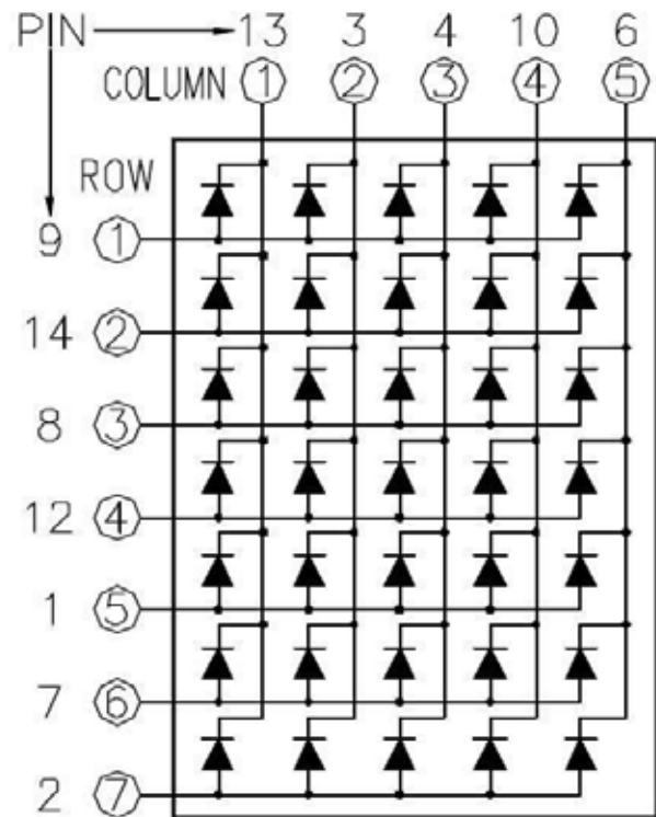
CDMC5712 SERIES (COLUMN CATHODE)
