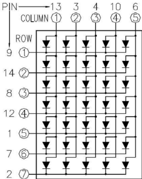
CDMA5712 SERIES (COLUMN ANODE)
